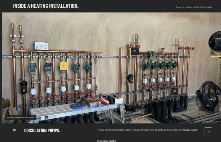
Numbered details explain a heating installation.
